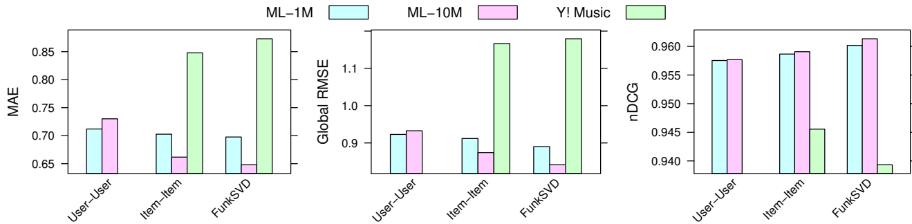
Figure 3: Representative algorithms
